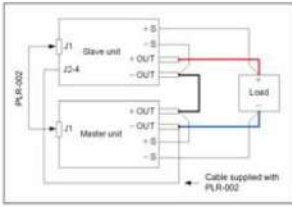
Series Connection Diagram
